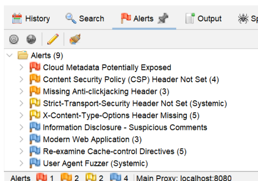
Gambar 5. Hasil Scan ZAP SMK At-Tamimi
