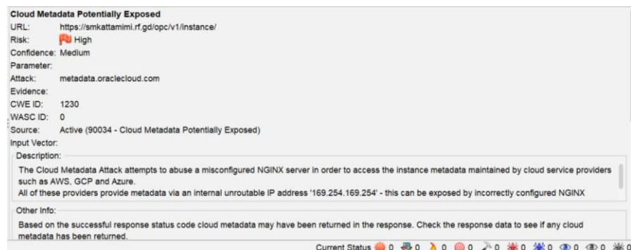
Gambar 6. Indikasi alert Cloud Metadata Potentially Exposed
