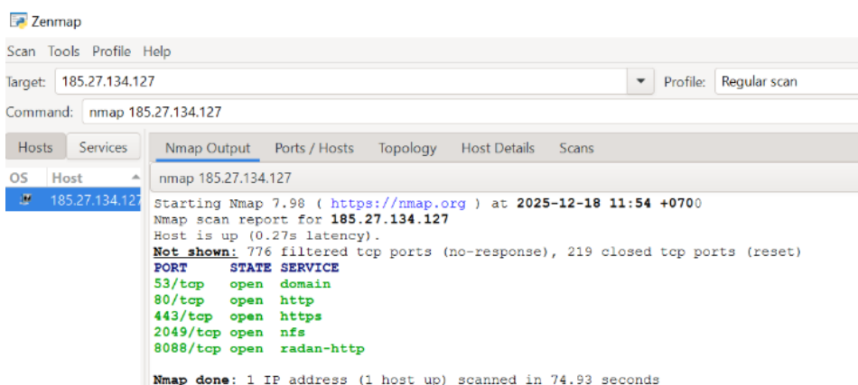
Gambar 4. Hasil Scan Zenmap GUI SMK At-Tamimi
